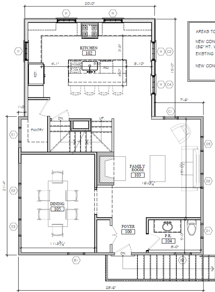
2 PROPOSED FIRST FLOOR PLAN SCALE: 1/4" = 1'-0"
