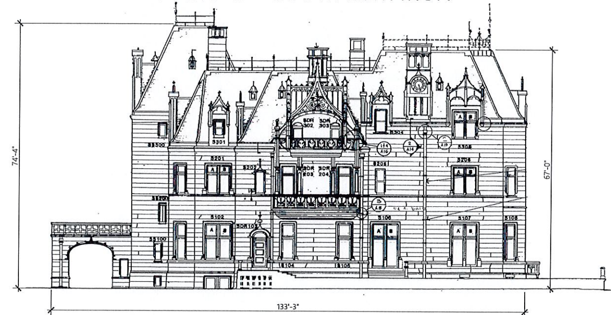
OCHRE COURT - SOUTH ELEVATION
