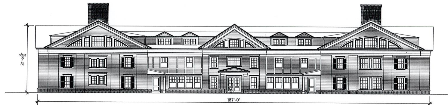
BUILDING "A" - NORTH ELEVATION
